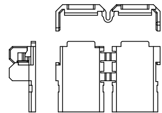
Cable Clamp
